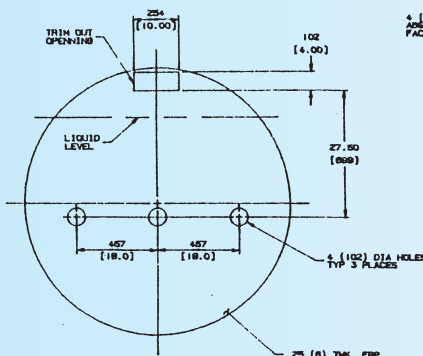
DIVIDER PANEL
